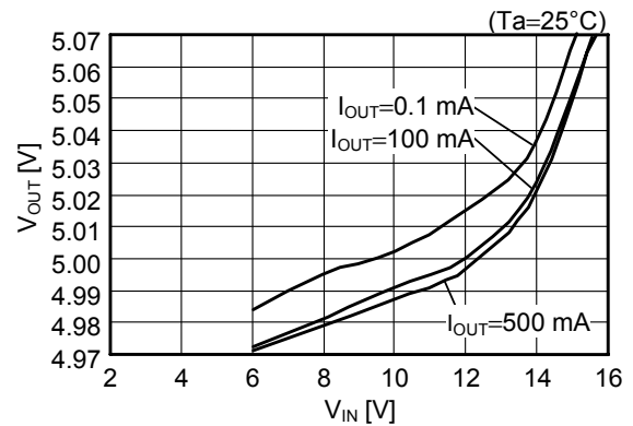
S-8521F50MC
