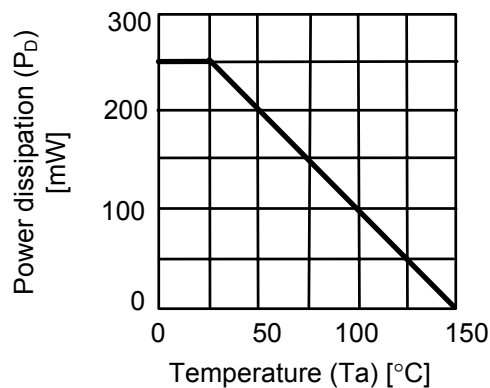
Figure 4 Power dissipation of Package (Before mounting)
