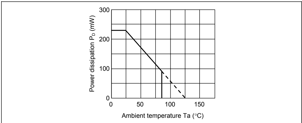
Figure 3 Power dissipation of package
